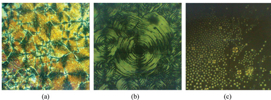
Figure 3. Textures of investigated compounds in cooling: a) Mix7 – polygonal texture at 70^\circ\text{C} ; b) Mix5 – circular texture at 60^\circ\text{C} ; c) Mix 5 – growth of spherulites from the isotropic phase at 80^\circ\text{C} . (Figure appears in color online.)
