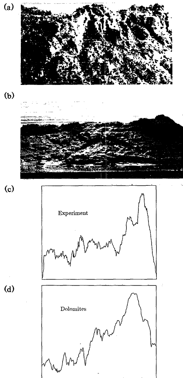
FIG. 1. (a),(b) Two representative morphologies obtained by spraying the model ridges of length 65 cm for 20 and 10 min, respectively. In (c) we display the digitized and rescaled (reduced in the horizontal direction by a factor of 4) image obtained from the profile of the picture in (b). (d) For comparison the digitized profile of one of the mountains in the Dolomites is also shown.
