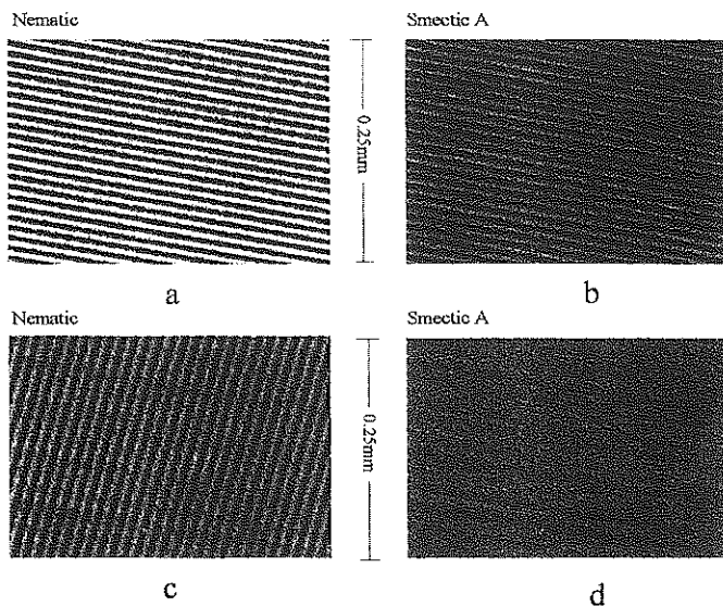
FIGURE 5 Periodic structures induced by the polarization grating. a and b: the grating vector perpendicular to rubbing direction at 37.2^{\circ}\text{C} and 31^{\circ}\text{C} respectively; c and d: the grating vector parallel to rubbing direction at 37.2^{\circ}\text{C} and 31^{\circ}\text{C} respectively.
