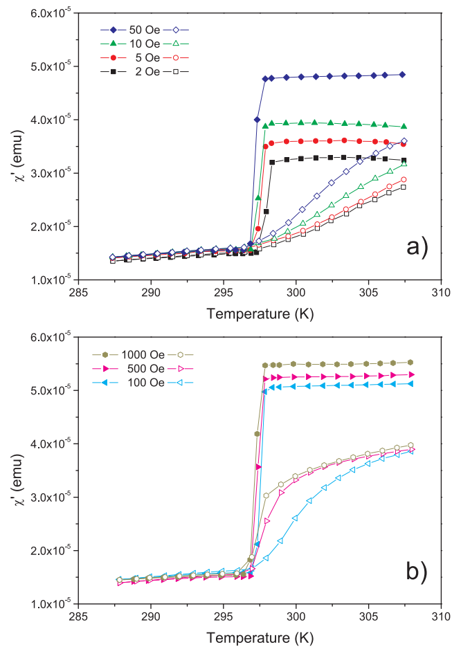
Fig. 1. Temperature dependence of the real part \chi' of the ac susceptibility for the sample with the volume concentration \phi_1 = 5 \times 10^{-4} in a cooling-heating cycle, with a prior application of a dc biasing magnetic field as indicated in the legend. Solid and open symbols correspond to the data obtained on cooling and in heating, respectively.
