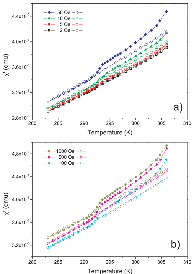
Fig. 2. Temperature dependence of the real part \chi' of the ac susceptibility for the sample with the volume concentration \phi_2 = 10^{-3} in a cooling-heating cycle, with a prior application of a dc biasing magnetic field as indicated in the legend. Solid and open symbols correspond to the data obtained on cooling and in heating, respectively.
